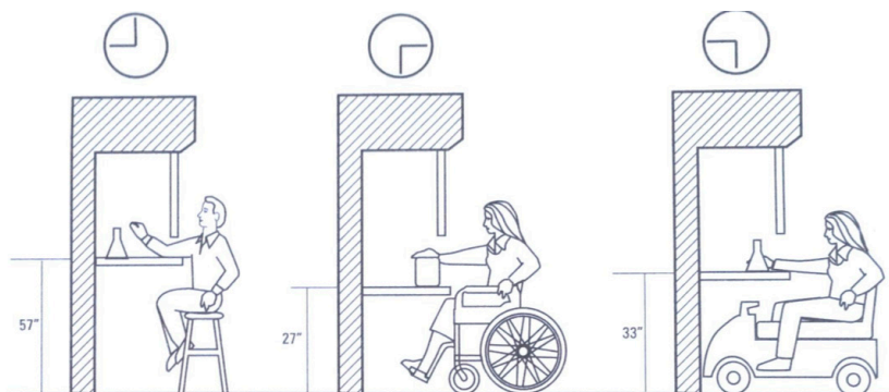
Fume hood clearances
